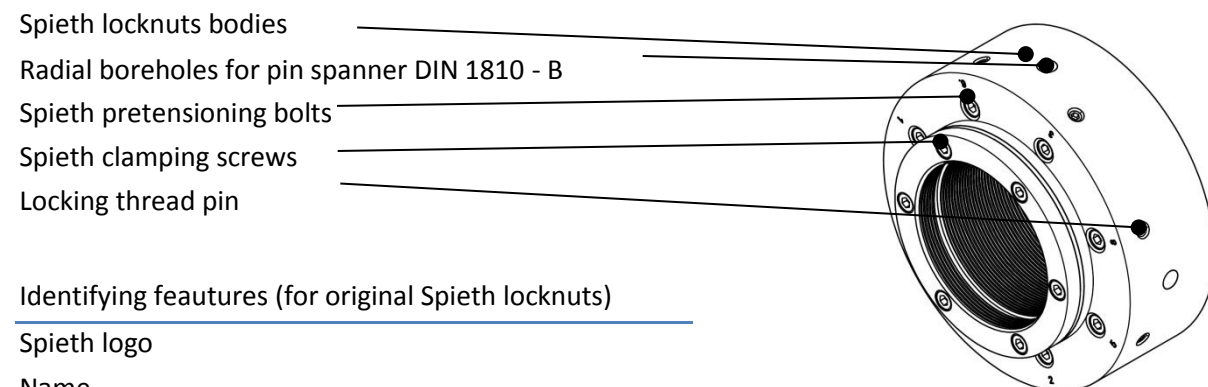
Fig 1: Schematic representation similar to Spieth MSW series locknuts
